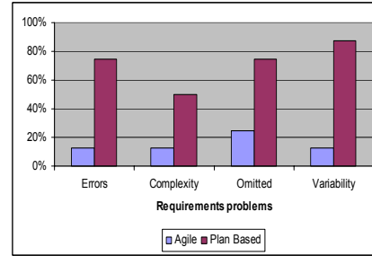
Figure 2: Requirements problems
