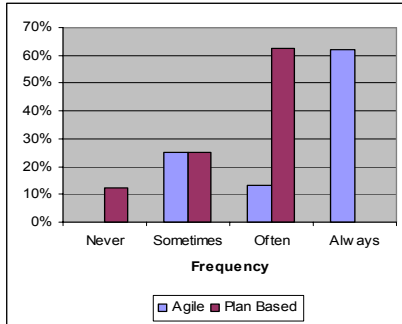
Figure 1: Frequency of requirements variability
