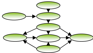
Deployment Model
