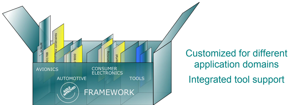
Agile Framework
